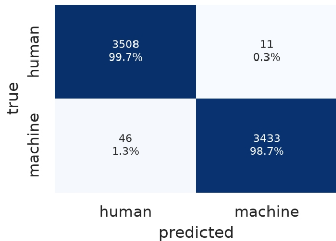
SGD [hinge] char3-5, F1=0.9919
