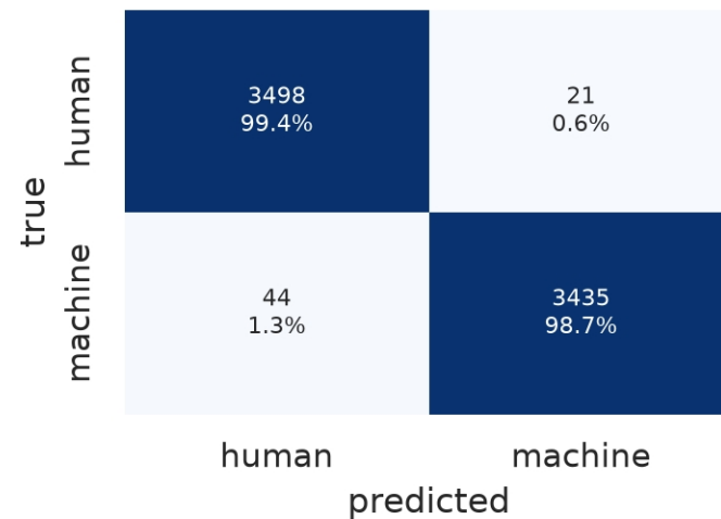
PassiveAggressive TF-IDF, F1=0.9907
