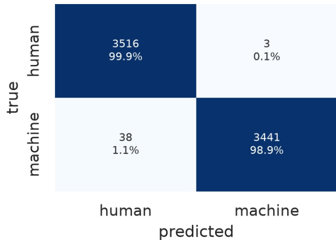
RidgeClassifier char3-5, F1=0.9941
