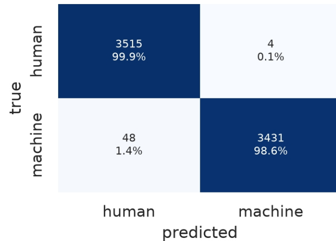
LightGBM TF-IDF-s, F1=0.9926
