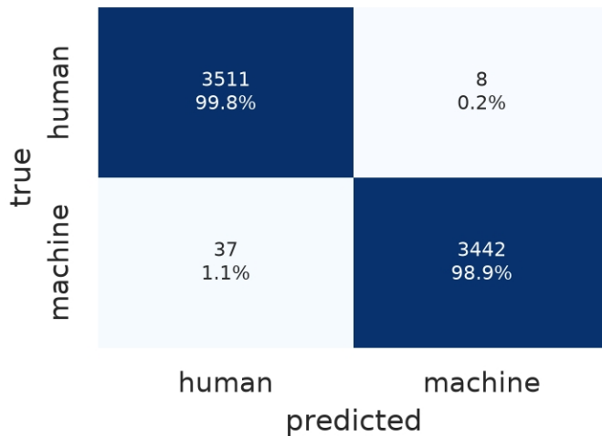
LinearSVC char3-5, F1=0.9936
