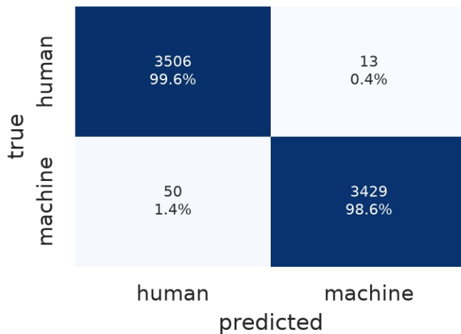
MLP [adam] TF-IDF-s, F1=0.9910
